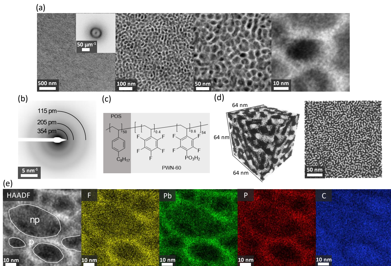
Figure 3: Nanophase separation in POS-b-PWN-60. (a) HAADF-STEM images of Pb 2+ stained membrane cross-section and diffractogram for nanostructure size determination. (b) Mean atomic-bond lengths from SAED. (c) Chemical structure of the polymer from synthesis. (d) Nanophase simulation of POS 50 -b-PWN-66 50 with the same parameters from Figure 1. Similar to (a), the dark parts correspond to the non-polar POS-rich phase. (e) Structure domains highlighted in HAADF image and corresponding EDXS images for fluorine, lead, phosphorus and carbon.
