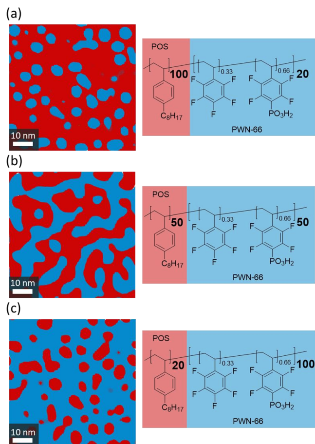
Figure 1: Mesostructure simulations of nanophase separation of POS-b-PWN-66 with block lengths of 100:20 (a), 50:50 (b), 20:100 (c). The simulated cubes consist of 5543 (a), 7763 (b), 7769 (c) distinct POS-b-PWN-66 chains.
